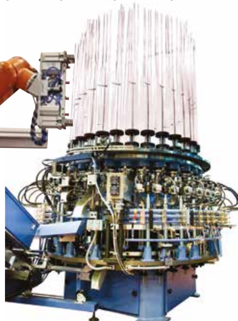
AMPOULE FORMING MACHINE MA30
